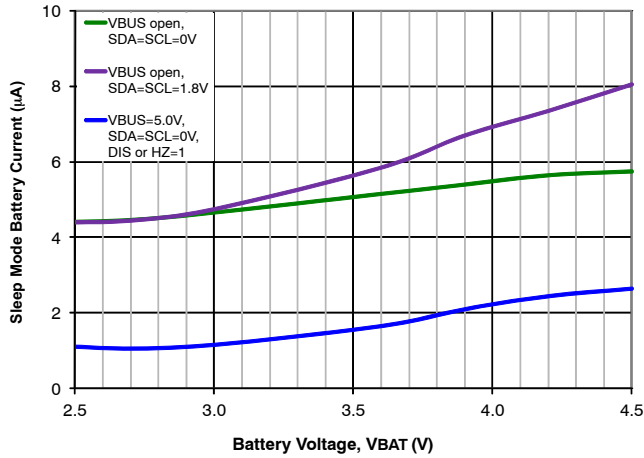
Figure 20. Battery Discharge Current vs. Mode
