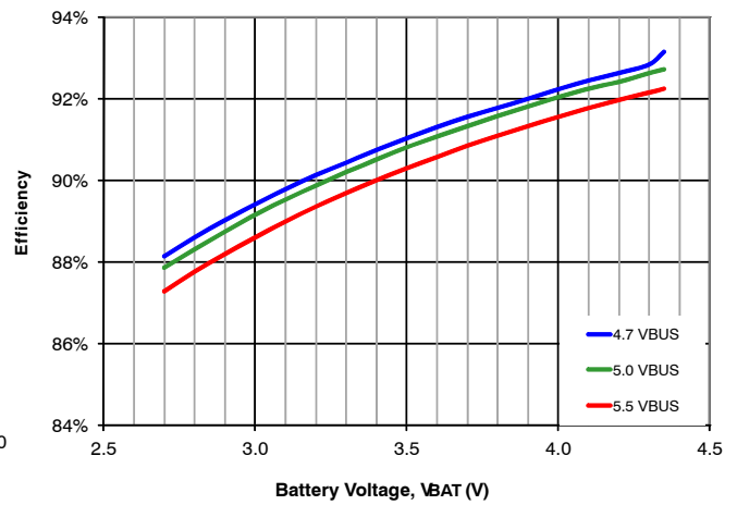
Figure 9. Charger Efficiency vs. V_{BAT} , I_{INLIM}=500\text{ mA} , V_{OREG}=4.35
