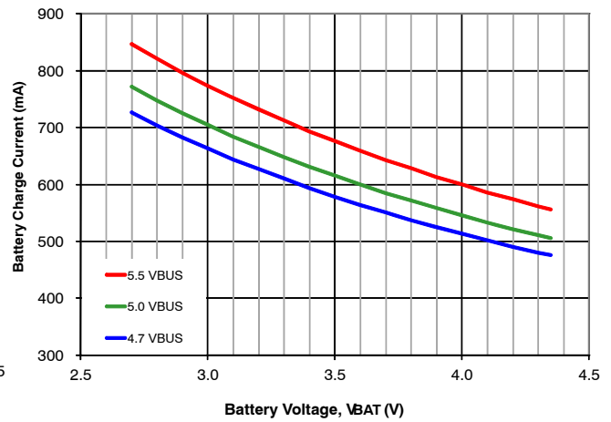
Figure 7. Battery Charge Current vs. V_{BAT} with I_{INLIM}=500\text{ mA} , V_{OREG}=4.35\text{V}
