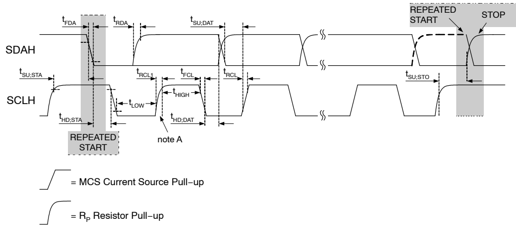
Figure 5. I²C Interface Timing for High-Speed Mode
