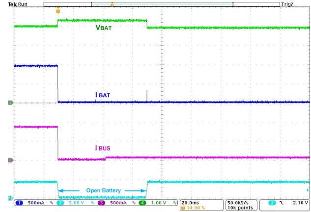
Figure 15. Battery Removal / Insertion During Charging, V_{BAT}=3.9 \text{ V} , I_{CHARGE}=1050 \text{ mA} , No I_{INLIM} , TE=1
