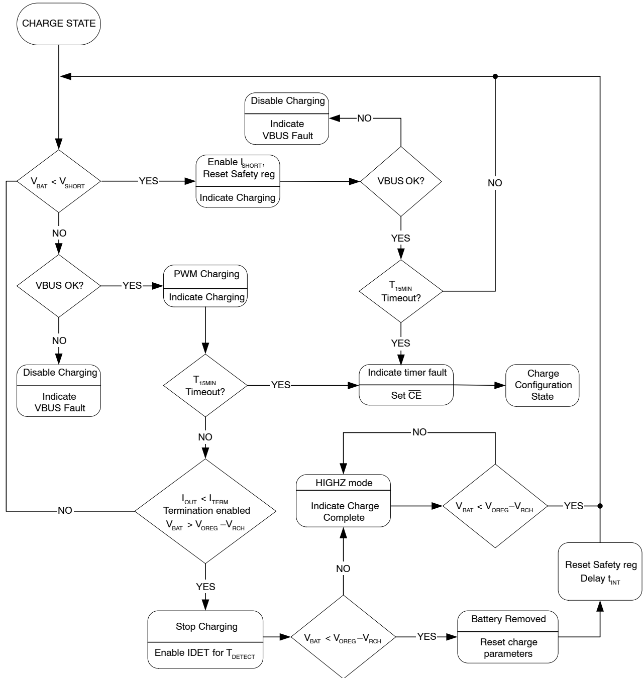
Figure 37. Charge Mode
