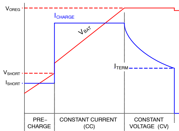
Figure 34. Charge Curve, I CHARGE Not Limited by I INLIM
