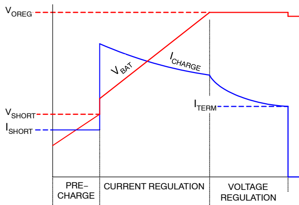
Figure 35. Charge Curve, I INLIM Limits I CHARGE
