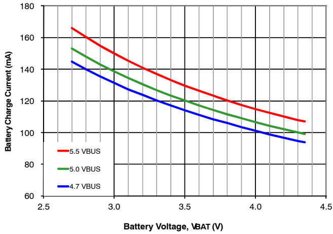
Figure 6. Battery Charge Current vs. V_{BAT} with I_{INLIM}=100\text{ mA} , V_{OREG}=4.35\text{V}
